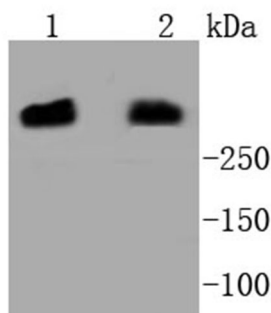
Fig. 1. Western blot analysis of DNA PKcs on different lysates using anti-DNA PKcs antibody at 1/1,000 dilution. Positive control: Lane 1: HeLa; Lane 2: MCF-7
